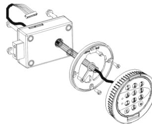
System with spindle variant B
