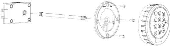
System with spindle variant A
